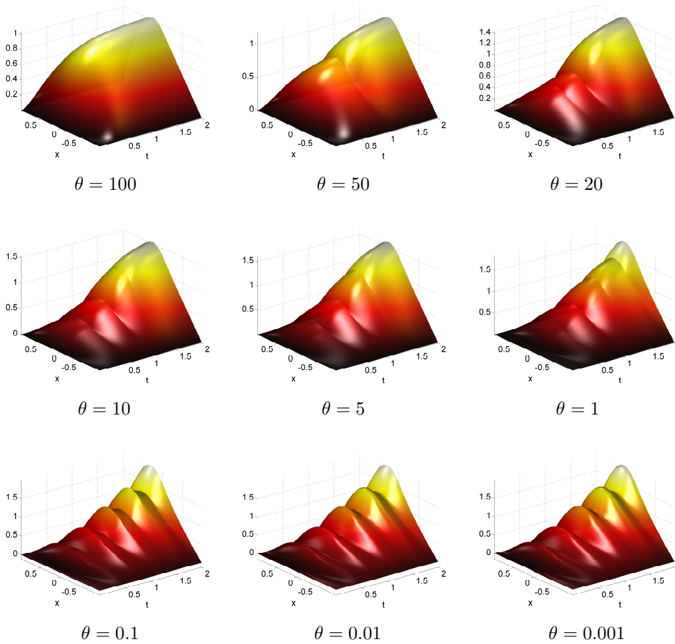
FIG. 3. Example 1: \bar{y}_\sigma^\theta for different values of \theta .
