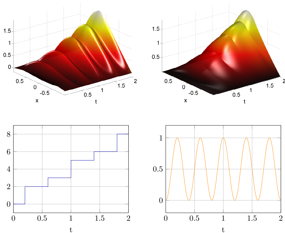
FIG. 1. Example 1: y_{d,\sigma} and \bar{y}_\sigma (top left and right), \bar{u}_\tau and \bar{\lambda}_\tau (bottom left and right).
