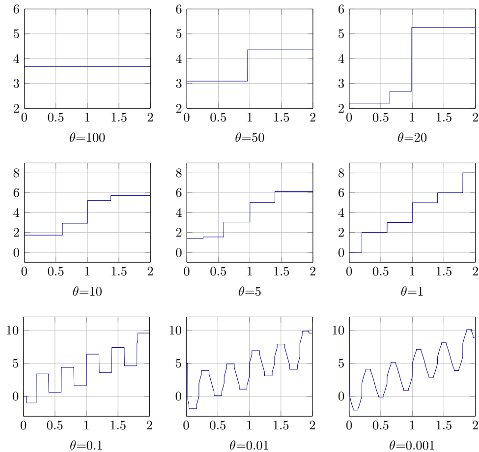
FIG. 4. Example 1: \bar{u}_\tau^\theta for different values of \theta .
