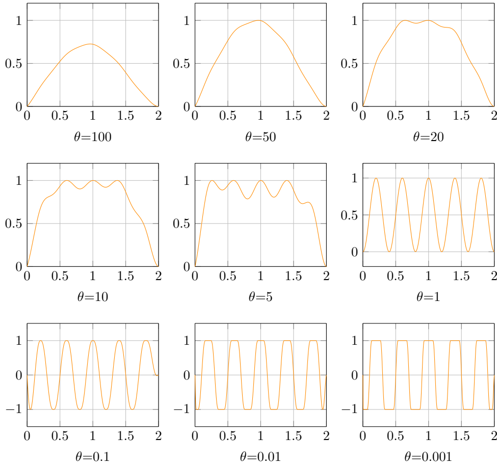
FIG. 5. Example 1: \bar{\lambda}_\tau^\theta for different values of \theta .
