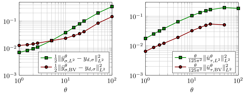
FIG. 6. Example 1: \bar{u}_{\tau, L^2}^\theta for different values of \theta .
