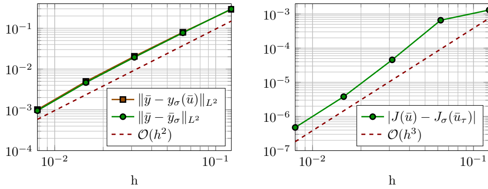
FIG. 2. Example 1: Discretization errors for optimal state and optimal objective value.
