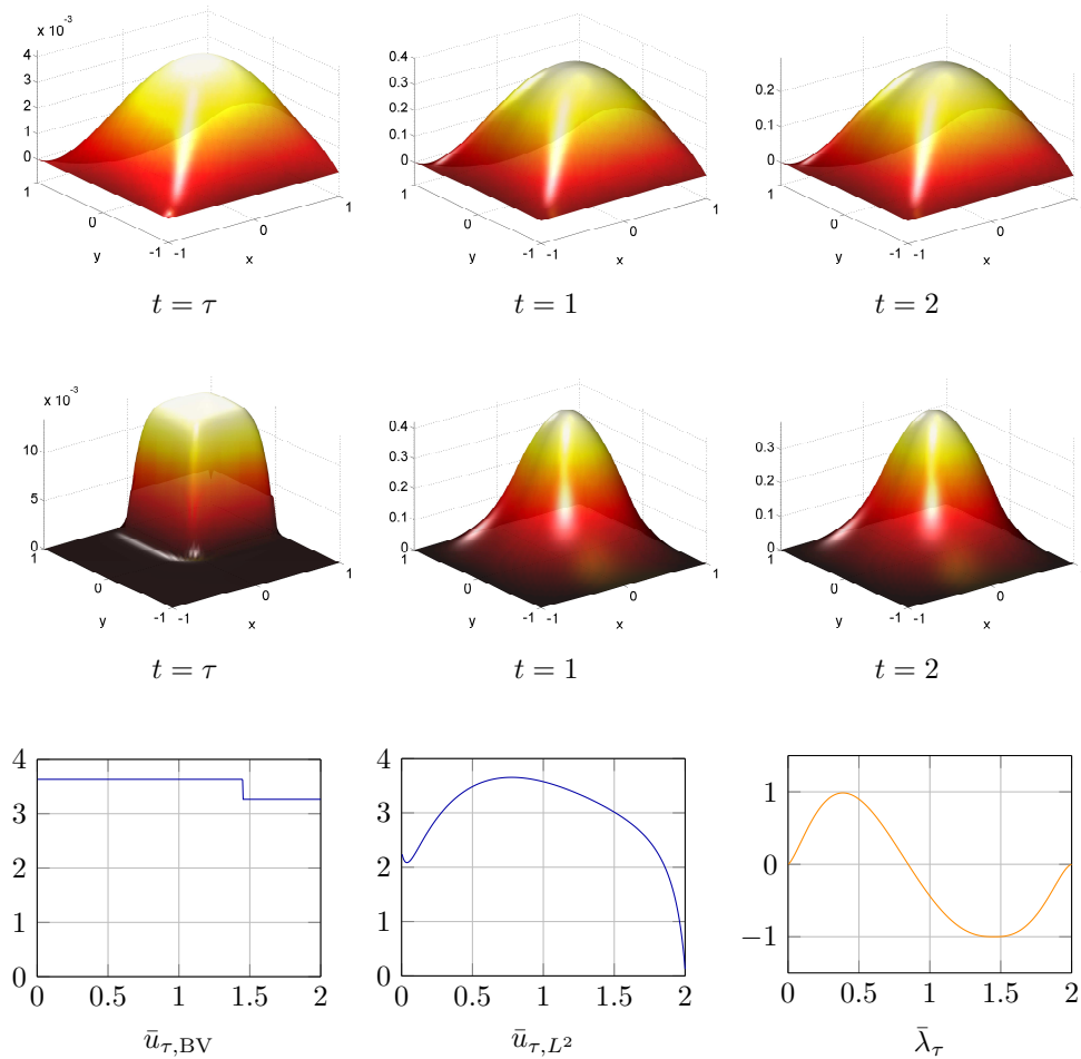
FIG. 9. Example 3: y_{d,\sigma} (top) and \bar{y}_\sigma (middle) for different t , \bar{u}_{\tau, BV} , \bar{u}_{\tau, L^2} , and \bar{\lambda}_\tau .
