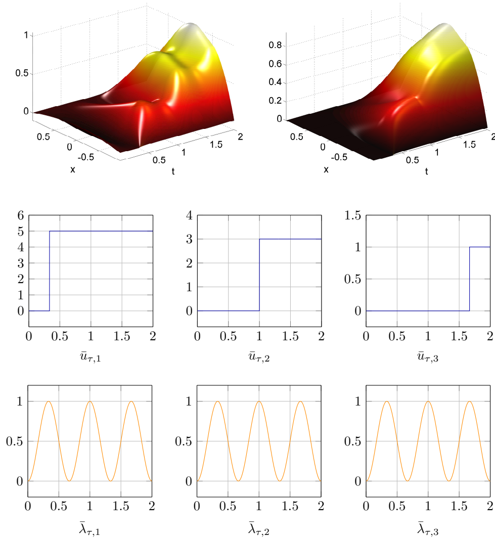
FIG. 8. Example 2: y_{d,\sigma} and \bar{y}_\sigma (top left and right), (\bar{u}_{\tau,j})_j , and (\bar{\lambda}_{\tau,j})_j .
