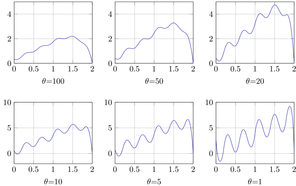
FIG. 6. Example 1: \bar{u}_{\tau, L^2}^\theta for different values of \theta .
