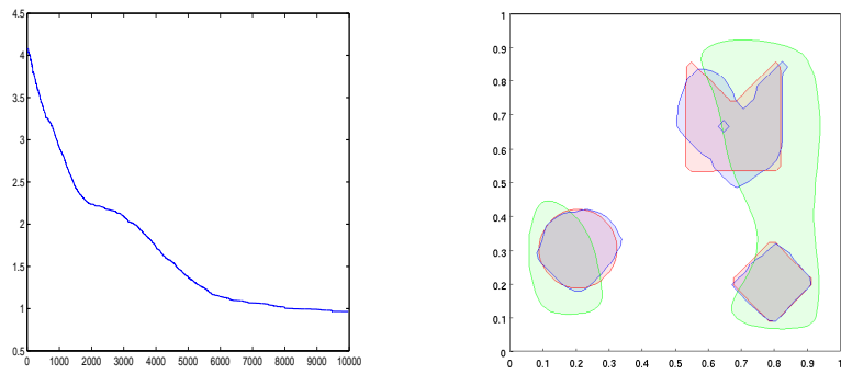
FIGURE 3. Second example after 10000 iterations. Left: Conductivity q_1 over the iterations. Right: Initial domain \Omega_1 after topological sensitivity (green); final domain \Omega_1 upon termination of the algorithm (blue); true domain \Omega_1 (red).
