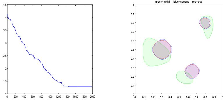
FIGURE 2. First example after 2000 iterations, with 1% noise. Left: Conductivity q_1 over the iterations. Right: Initial domain \Omega_1 after topological sensitivity (green); final domain \Omega_1 upon termination of the algorithm (blue); true domain \Omega_1 (red).
