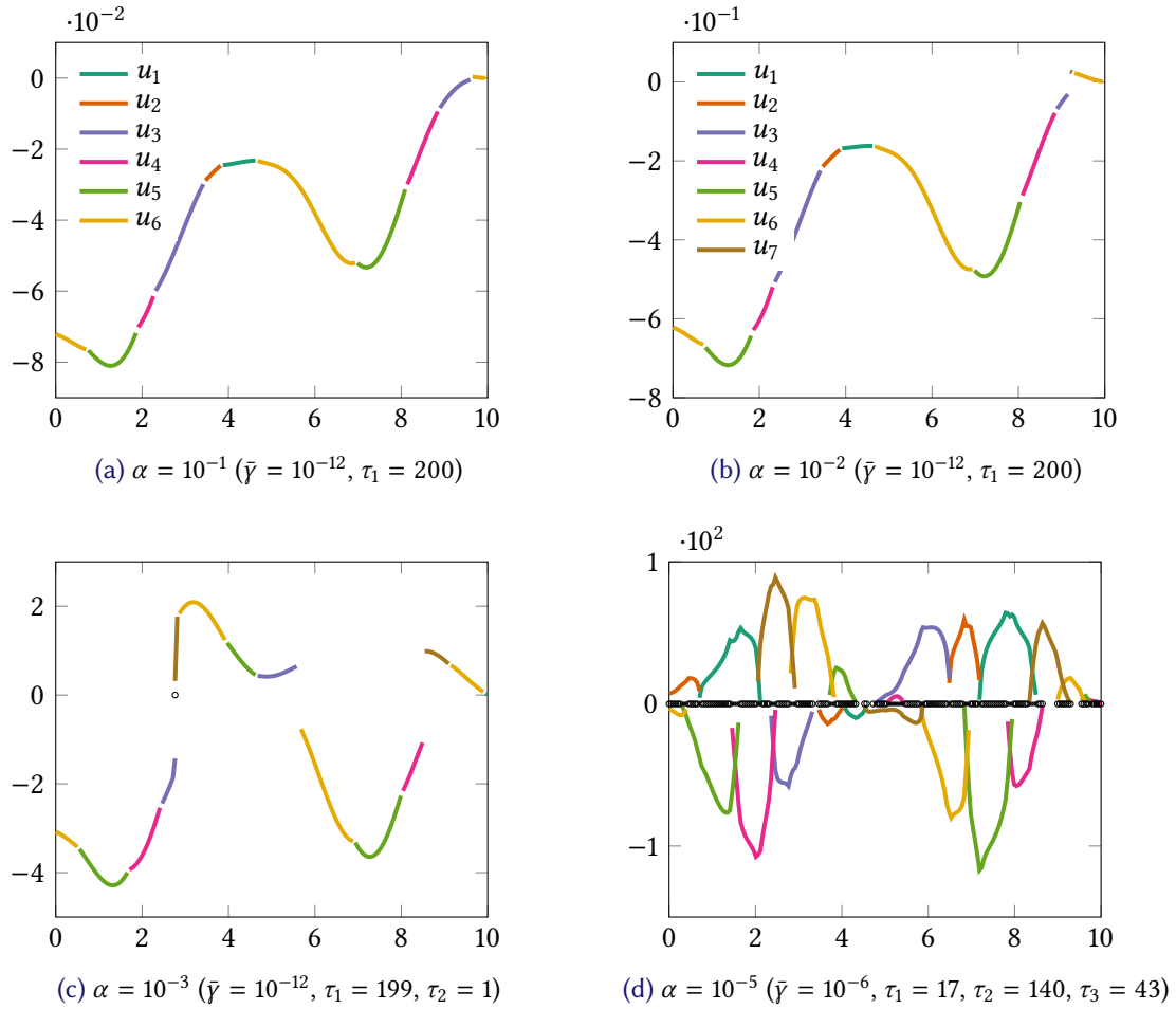
Figure 3: Dependence of the controls on \alpha for N = 7 . Control intervals without perfect switching are marked on the t -axis
