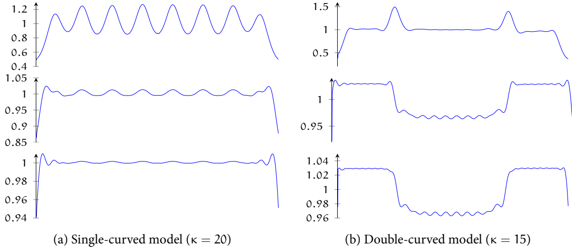
Figure 4: Photon densities \phi_\gamma (in \text{W m}^{-2} , normalized to unit mean) plotted along part of the observation region (left line in Fig. 1) for representative single-curved and double-curved models for three different values of alpha (from top to bottom: \alpha = 0.1 , \alpha = 0.01 , \alpha = 0.001 ).
