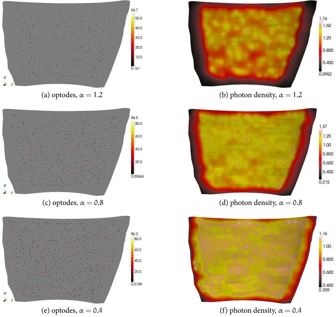
Figure 5: Optode positions and magnitudes (left) and photon densities (right; in \text{W m}^{-2} , normalized to unit mean) for the three-dimensional model and three different values of \alpha .
