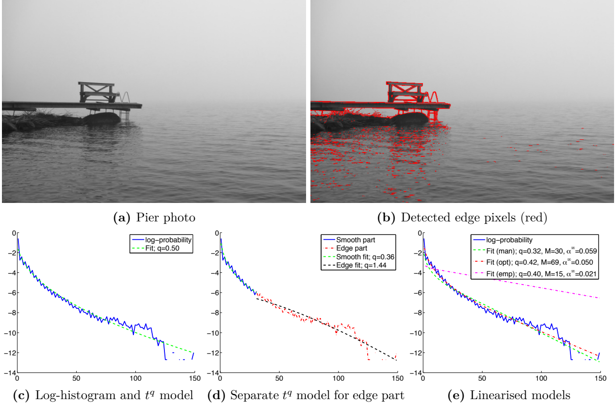
Figure 1: Pier photo: discrete gradient histogram and least squares models. The image intensity in (a) is in the range [0, 255] , and we have chosen pixels k with |\nabla u(k)| \geq 30 as edges (b). The log-histogram of |\nabla u(k)| with optimal fit of t \mapsto t^q is displayed in (c). This is done separately for the edge pixels in (d). The linearised model is fitted in (e) for the cut-off point M = 30 (manual edge detection), M = 69 (optimal least squares fit). We moreover show the empirically best linearised model.
