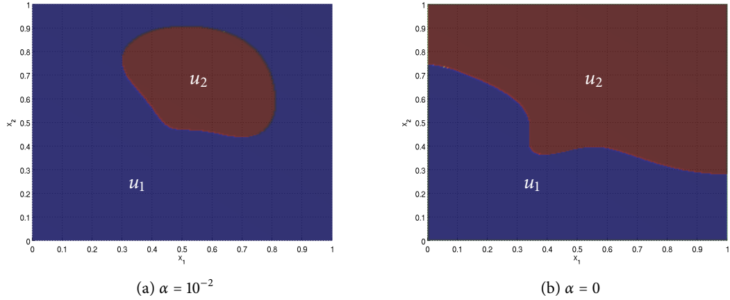
Figure 6: Comparison of multi-bang ( \alpha > 0 ) and bang-bang ( \alpha = 0 ) controls for (u_1, u_2) = (-1, 2) (shown are level-sets \{u_\varepsilon(x) = u_i\} )
