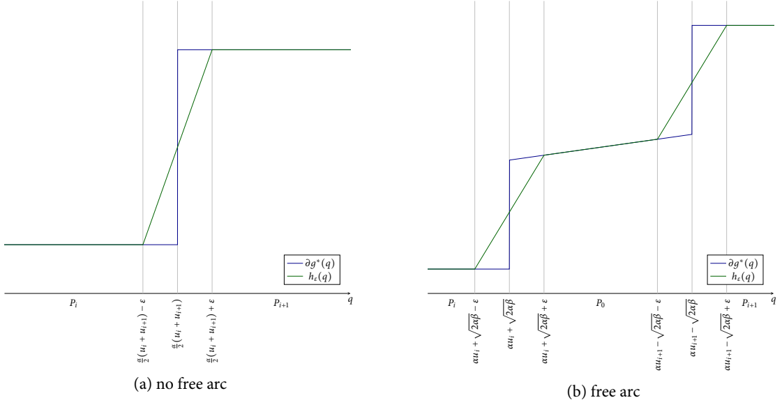
Figure 2: Possible situations for \partial g^*(q) and its regularization h_\varepsilon(q) . Left: \bar{P}_i \cap \bar{P}_{i+1} \neq \emptyset ; right: \bar{P}_i \cap \bar{P}_{i+1} = \emptyset and hence \bar{P}_i \cap \bar{P}_{i,0+} \neq \emptyset , \bar{P}_{i+1} \cap \bar{P}_{i+1,0-} \neq \emptyset
