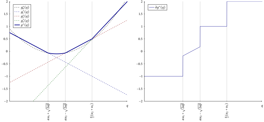
Figure 1: Plot of g^*(q) (left) and \partial g^*(q) (right) for d = 3 , (u_1, u_2, u_3) = (-1, 1, 2) , \alpha = 0.5 , \beta = 0.1
