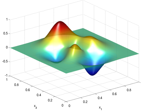
Figure 3: Target z for numerical examples
