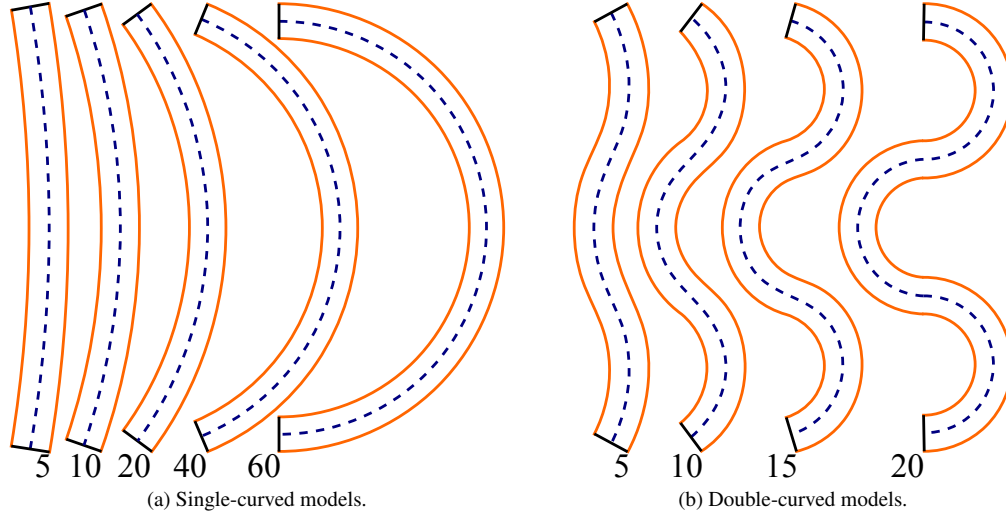
Fig. 1: Two-dimensional model geometries (numbers denote curvature \kappa ).
