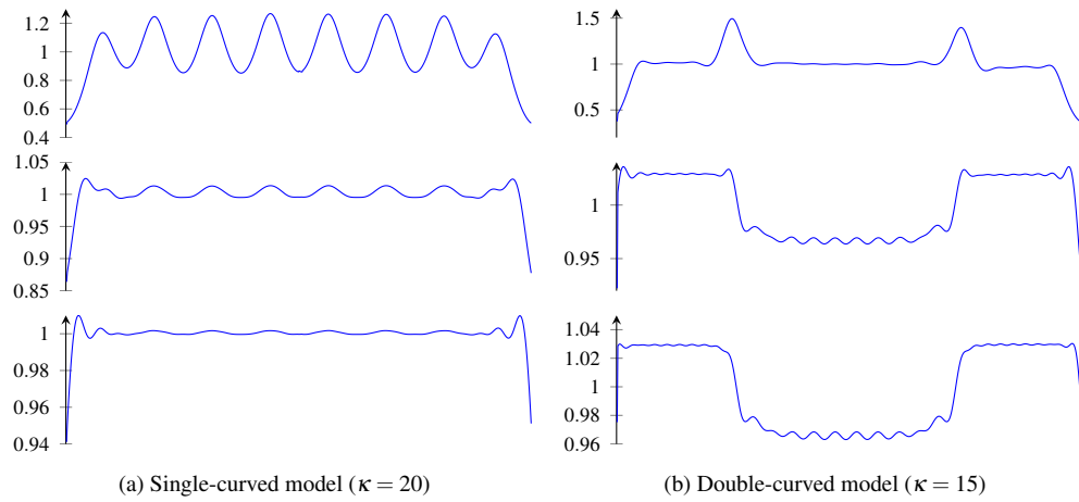
Fig. 4: Photon densities \phi_\gamma (in \text{W m}^{-2} , normalized to unit mean) plotted along part of the observation region (left line in Fig. 1) for representative single-curved and double-curved models for three different values of \alpha (from top to bottom: \alpha = 0.1 , \alpha = 0.01 , \alpha = 0.001 ).
