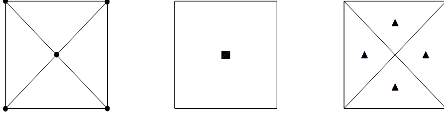
FIGURE 1. (cross-grid \mathbb{P}_1 )- \mathbb{Q}_0 elements. \bullet are the velocity nodes, \blacksquare are the pressure nodes and \blacktriangle are the multiplier nodes.
