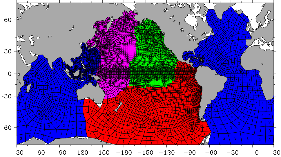
FIGURE 5.3. Northeast Pacific surface grid (NEP08) with 4 subdomains.
